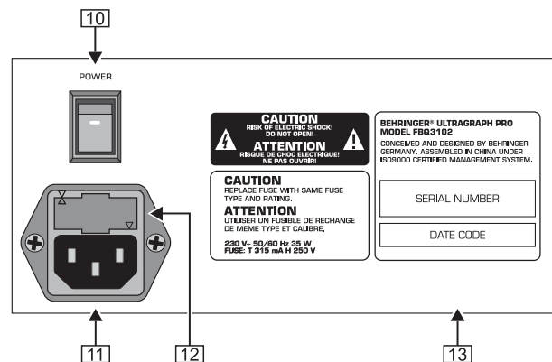
Fig. 2.2: Control elements and important information on the rear of the FBQ3102
