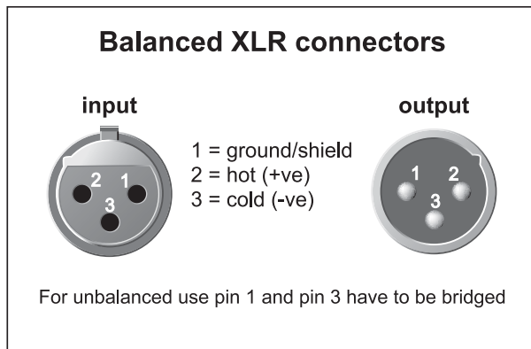
Fig. 4.1: XLR connectors
