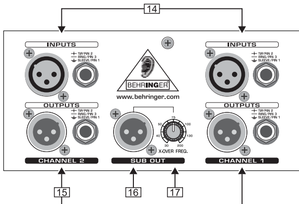
Fig. 2.3: Connectors at the rear of the FBQ3102
