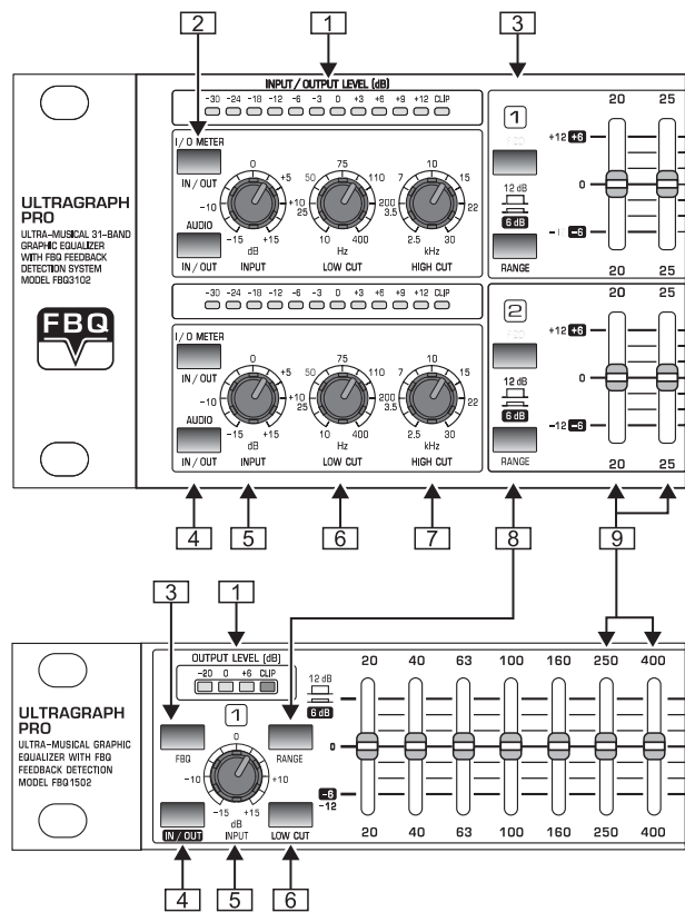
Fig. 2.1: Front panel control elements of the FBQ3102 (above) and of the FBQ1502 (below)
