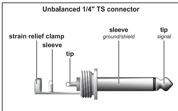
Fig. 4.2: 1/4" TS connector
