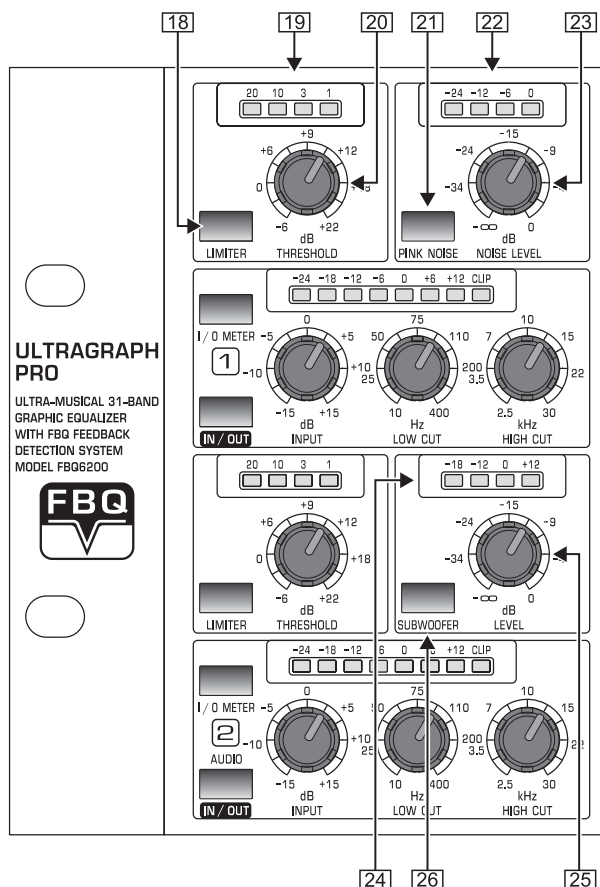
Fig. 2.4: FBQ6200 control elements
