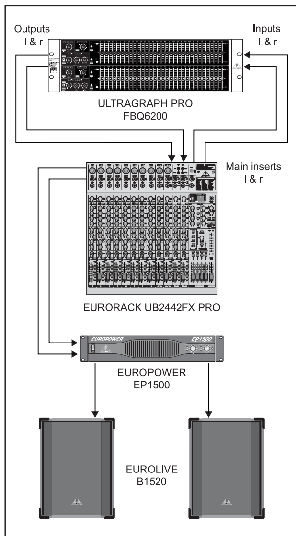
Fig. 3.1: The ULTRAGRAPH PRO FBQ6200 as master equalizer
